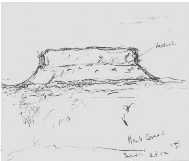
5a MOUNT CONNER, THE RED CENTRE, N.T.
